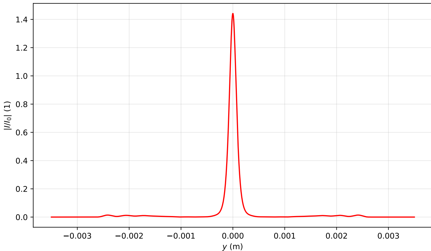
Intensity profile I(x=0, y, z=2.229)/I_0 , \text{Pin}=9.0\text{Pcr} , artificial time
